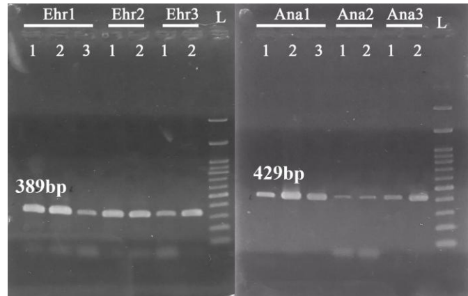
Fig. 1. Agarose gel electrophoresis of PCR products of 16S rRNA genes of Ehrlichia canis (left, 389bp) and Anaplasma platys (right, 429 bp). Ehr1, Ehr2 and Ehr3 for Ehrlichia and Ana1, Ana2, and Ana3 for Anaplasma are the sequences selected at random from pathogen-positive dog blood samples used for PCR. Each sample in the gel was used in either 2 or 3 technical replicates, shown here by the number under each well. The accession numbers are provided in the text. L is ladder
