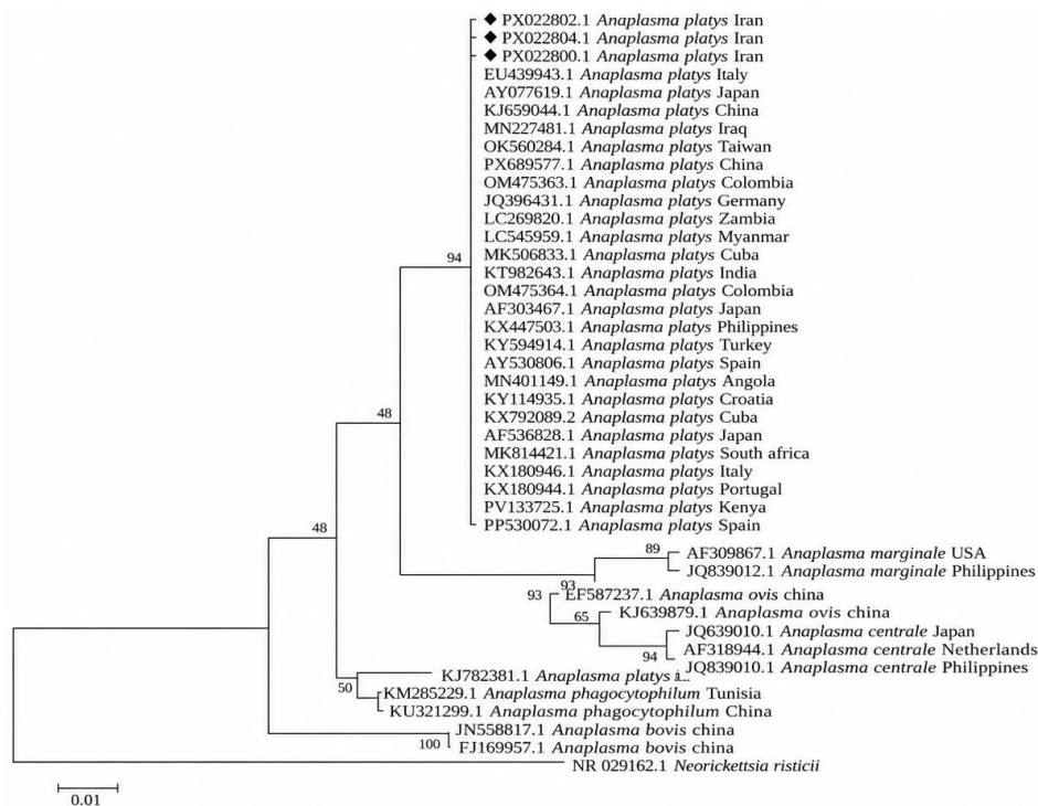
Fig. 5. Phylogenetic analysis of Anaplasma platys strains isolated in this study (marked with ♦) based on 16S rRNA sequences (429bp), compared to globally reported strains, using the Maximum Likelihood (ML) method with 1000 bootstrap replicates (Bootstrap support values are shown at the nodes) with the Tamura-Nei model. Neorickettsia risticii was used as the outgroup. GenBank accession numbers are shown. The scale bar represents 0.01 nucleotide substitutions per site
