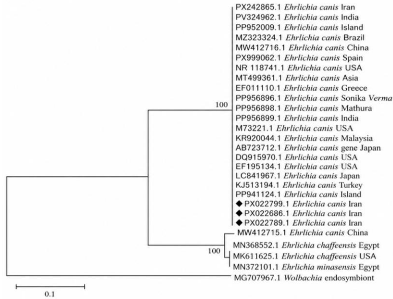
Fig. 4. Phylogenetic analysis of Ehrlichia canis strains isolated in this study (marked with ♦) based on 16S rRNA sequences (389bp), compared to globally reported strains, using the Maximum Likelihood (ML) method with 1000 bootstrap replicates (Bootstrap support values are shown at the nodes) with the Tamura-Nei model. Wolbachia endosymbiont was used as an outgroup. GenBank accession numbers are shown. The scale bar represents 0.1 nucleotide substitutions per site
