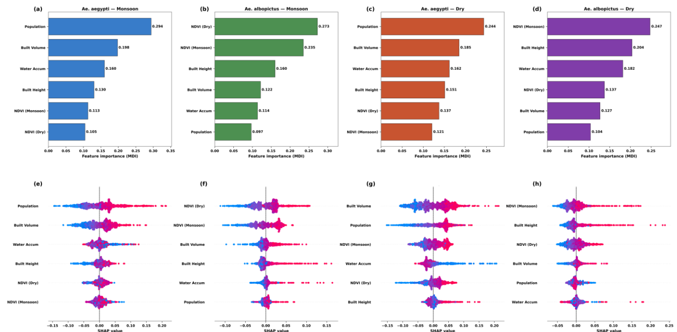
Fig. 3. Random Forest feature importance and SHAP beeswarm plots for environmental predictors of Aedes larval density in Bhopal, India (exploratory spatial analysis). The top row shows Mean Decrease in Impurity (MDI) feature importance for (a) Ae. aegypti monsoon, (b) Ae. albopictus monsoon, (c) Ae. aegypti dry season, and (d) Ae. albopictus dry season. The bottom row shows corresponding SHAP beeswarm plots for (e) Ae. aegypti monsoon, (f) Ae. albopictus monsoon, (g) Ae. aegypti dry season, and (h) Ae. albopictus dry season. See Supplementary Tables S3–S4 for the corresponding PLSR-VIP and LMG hierarchical-partitioning results
