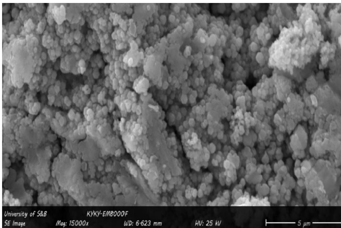
Fig. 1. Scanning electron microscopy of green-synthesized copper oxide nanoparticles (CuO NPs) showing surface morphology and aggregation; 15,000× magnification, 25 kV, scale bar: 5 μm
